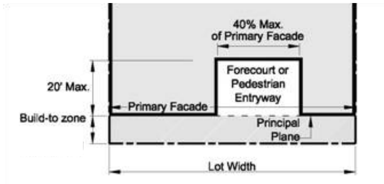
Figure 64-13-5.4 Forecourt Primary Facade Frontage
